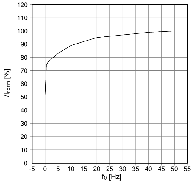
fo - derating curves IGBT (motor) cos(phi) = 0,85 T cool medium = 40°C
